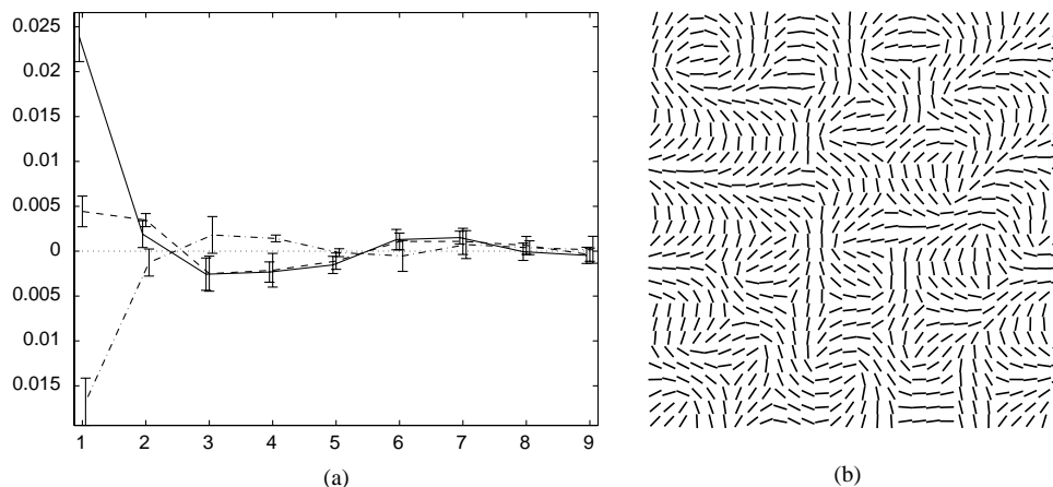
Fig. 2. (a) Swindale Kernels binned by distance ( \mu = 0.8 (- · -), 1.2 (- -), 1.6 (-)), as integrated for 4 maps for each \mu . (b) Resulting map produced using interaction kernel obtained from formation dynamics of the maps with high sparsity ( \mu = 1.6 ).
