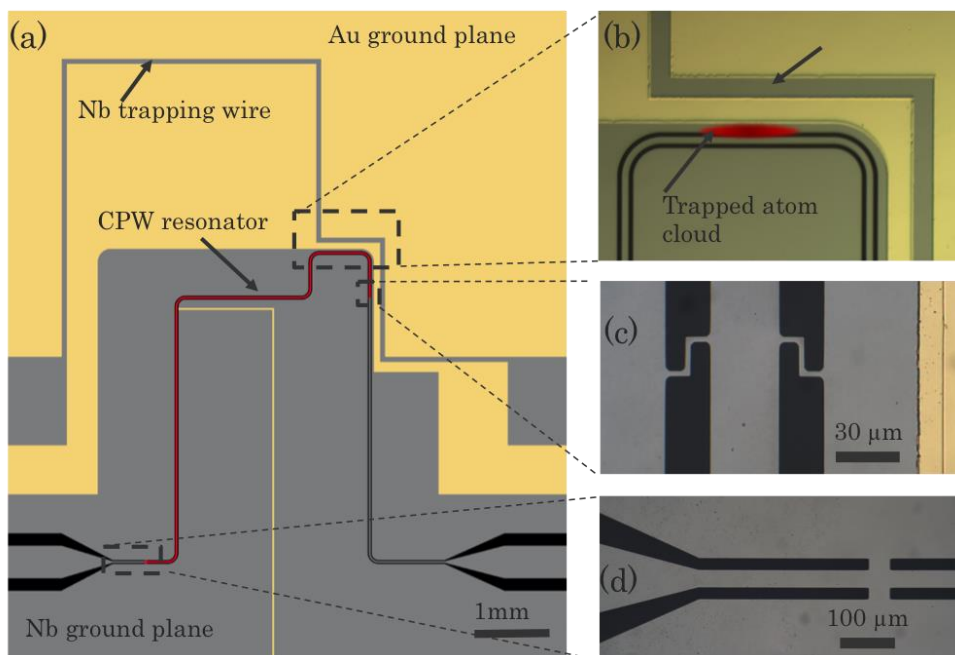
Graphic: Hybrid quantum architecture - Superconductor chip with captured atoms
